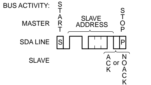
Figure 32. Software Write Protect (Read)
